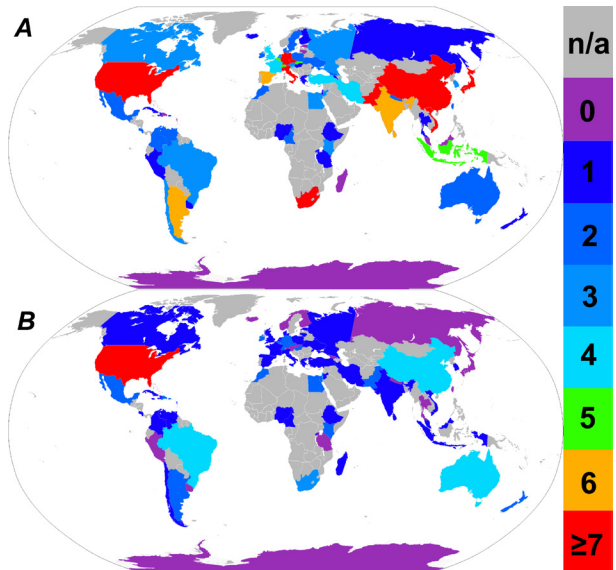
Fig. 1. Data on the distribution of Steinernema (A) and Heterorhabditis (B) in the world. The right column shows a relation between colors on map and number of species per country; "n/a" meaning: information is not available or research has not been carried out
